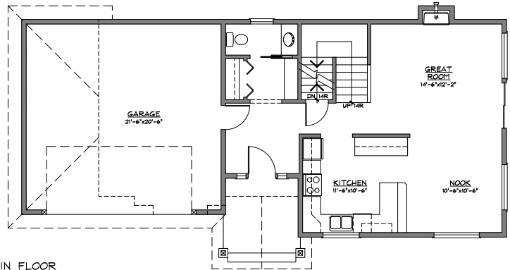
MAIN FLOOR 701 SF 701 SF (UNFINISHED BASEMENT) 430 SF (UPPER) 2332 SF TOTAL
